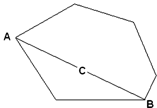
Figure 1. A visualization of “proof space”.
