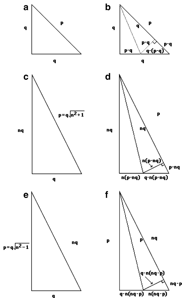
Figure 3. “Folding” proofs.
