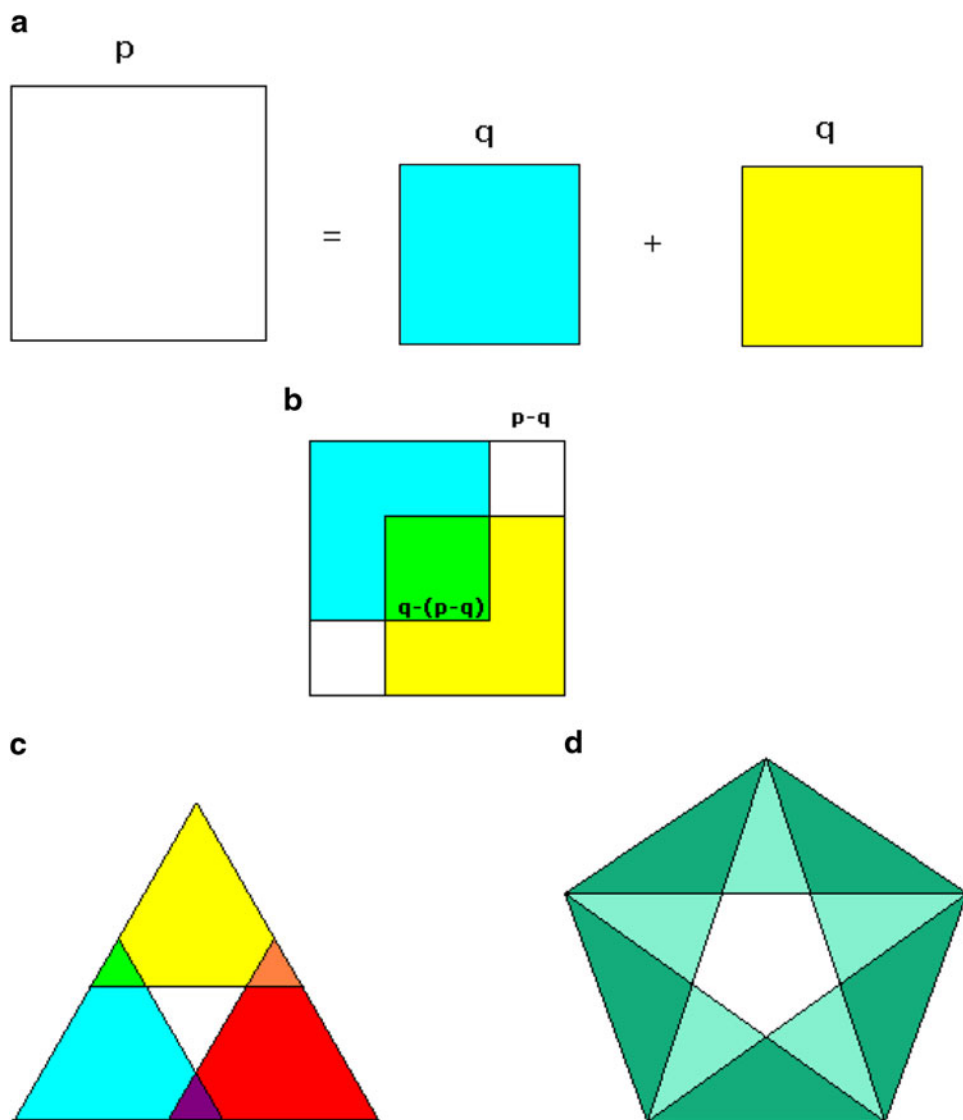
Figure 2. “Covering” proofs.
